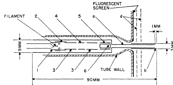
FIG. 2. Electron gun.
