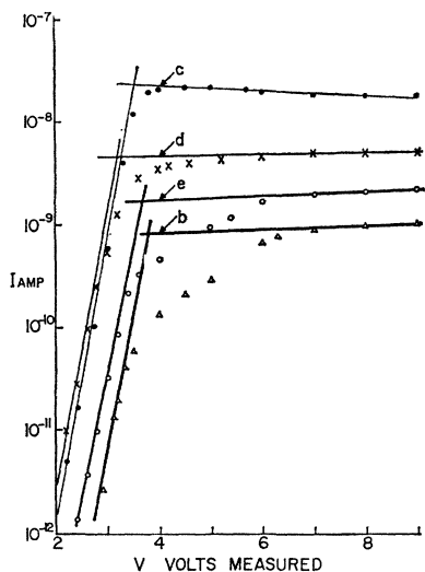
FIG. 3. Retarding field plots.
