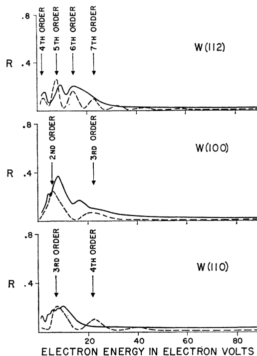
FIG. 16. Comparison between experimental results and prediction of the atomic model for reflection of slow electrons from three faces of tungsten. Solid lines: experiment; dashed lines: present model.
